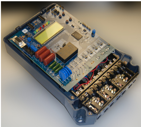
▲ EVM430-F6779 EVM
